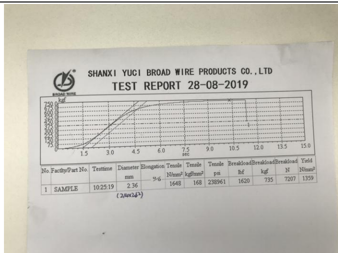
Result of tensile test
